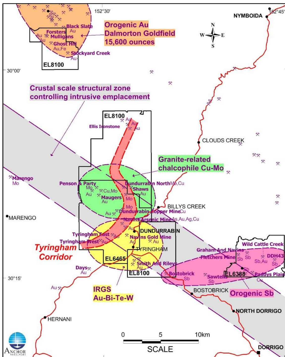
Figure 4: Blinks project structural architecture and metallogenes showing the Tyringham Corridor, inferred crustal suture zone and mineral occurrences
