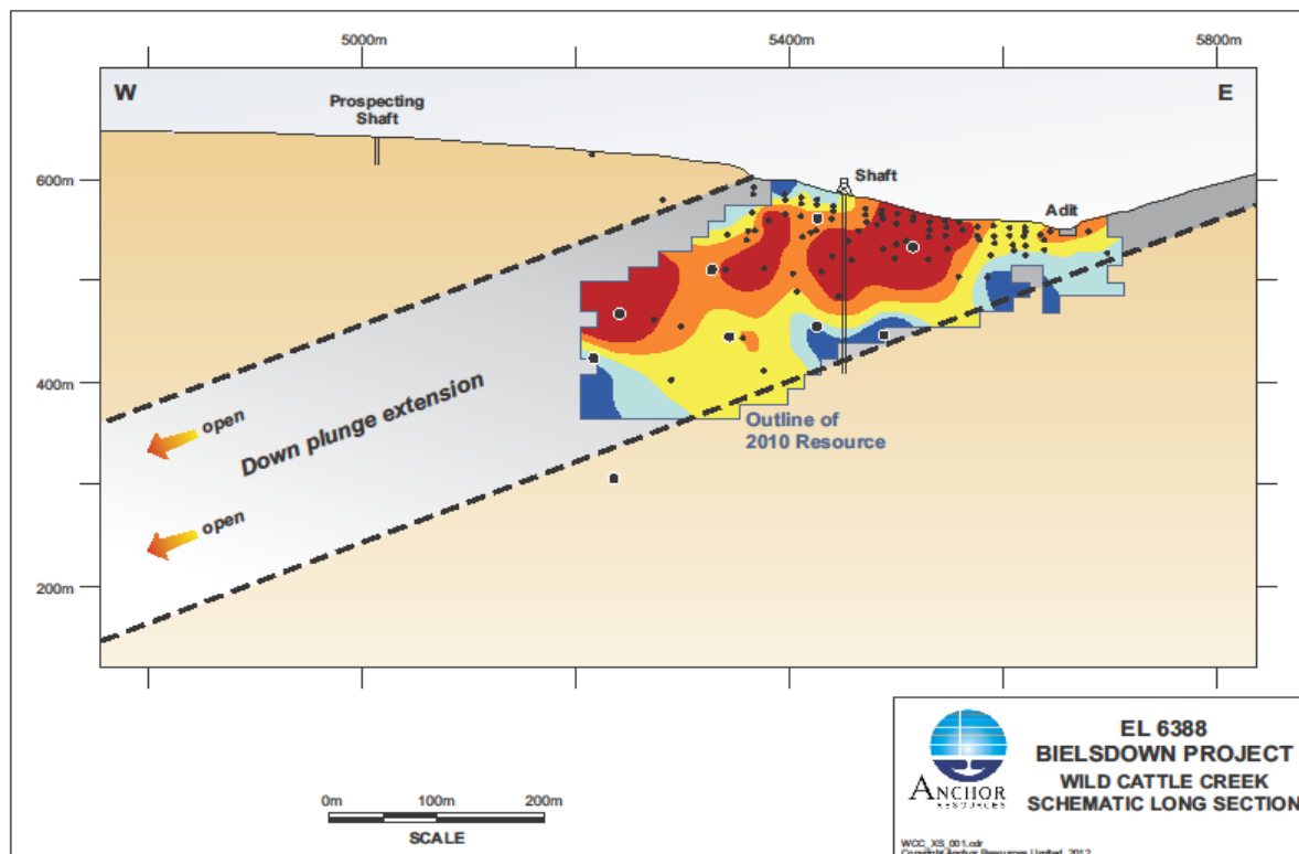
Figure 18: Bielsdown antimony deposit longitudinal section
