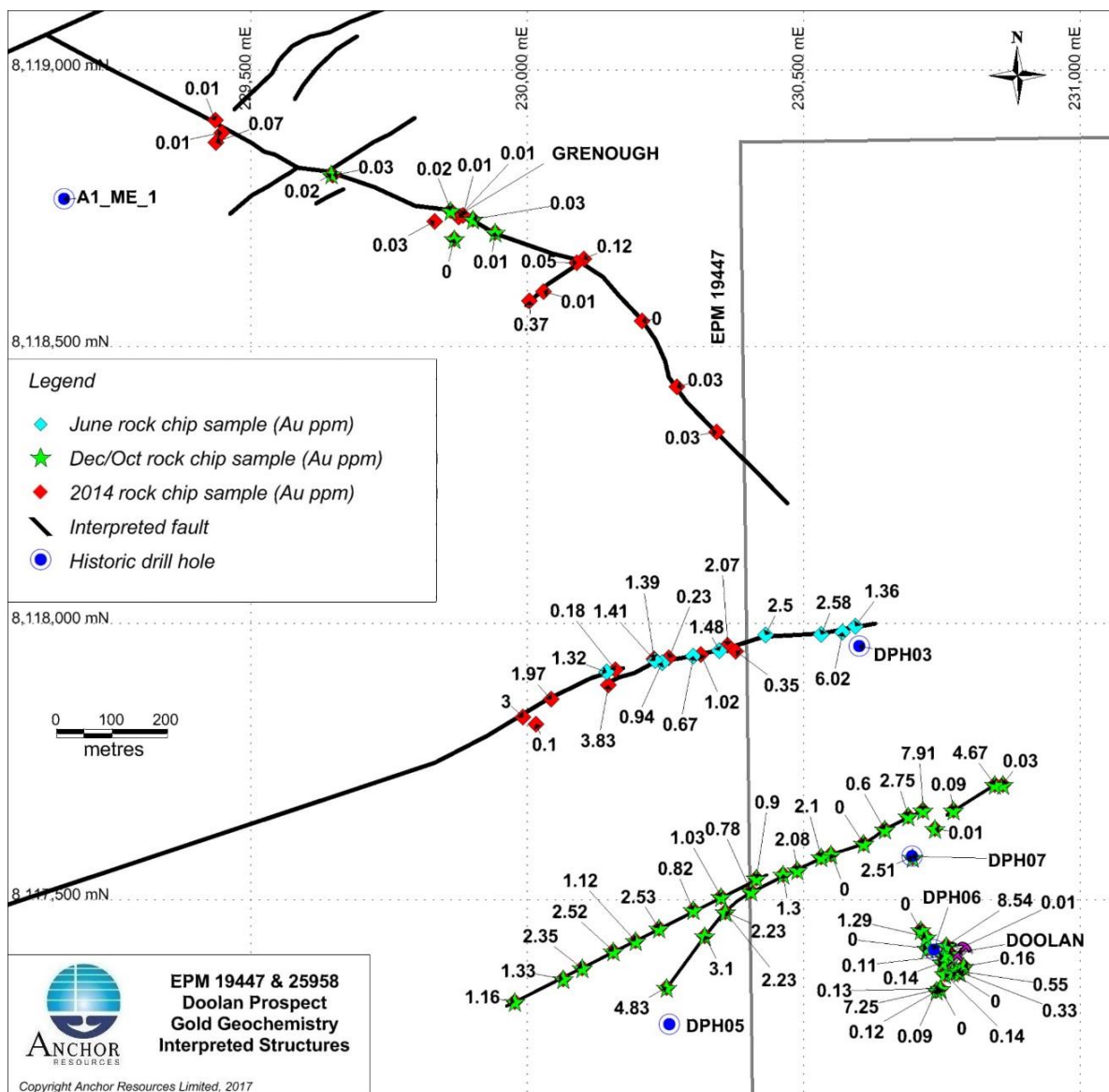
Figure 16: Doolan rock chip gold geochemistry
