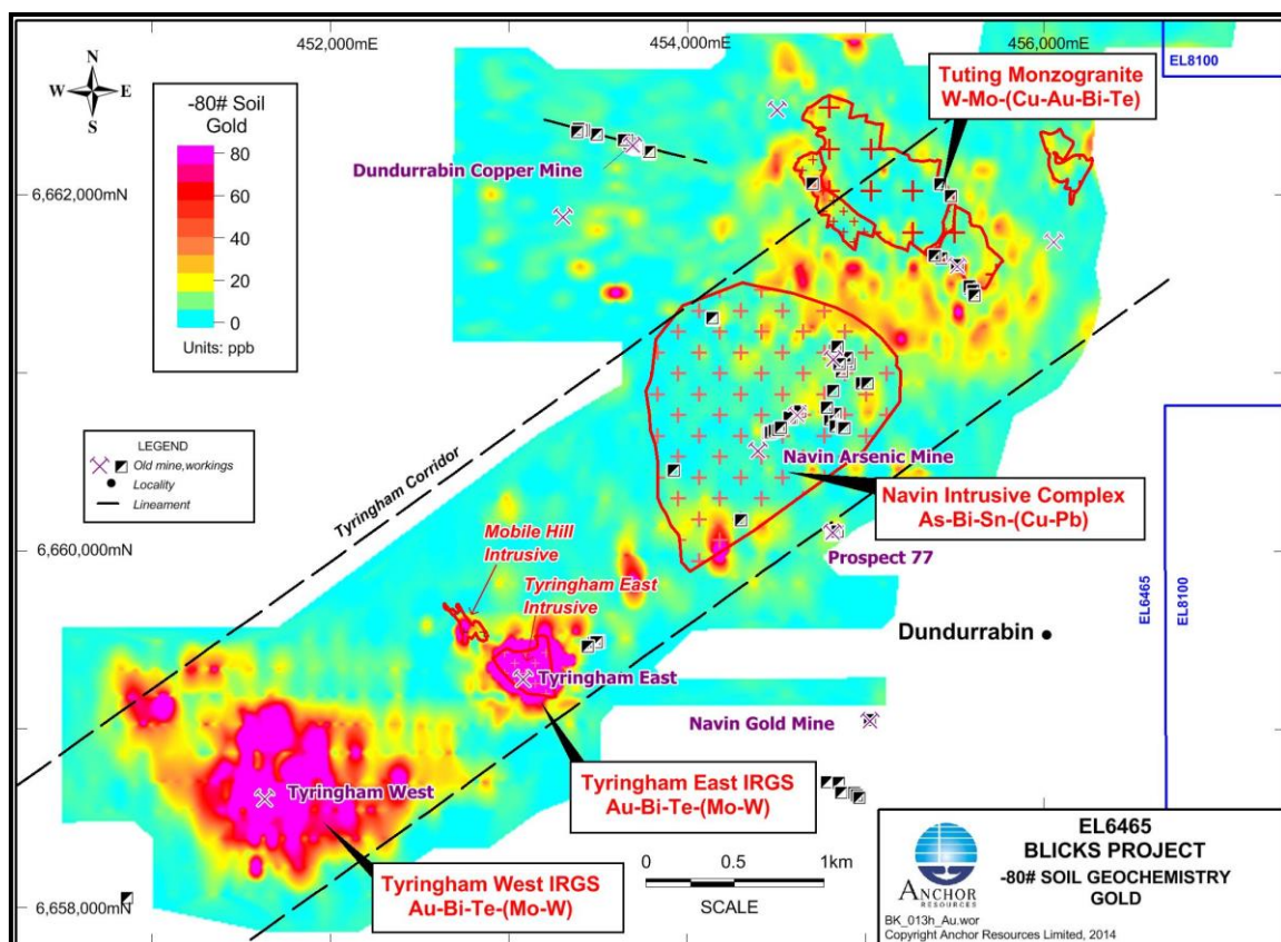
Figure 17 Tyingham Corridor – Gold in Soil (from Rabone, 2017)
