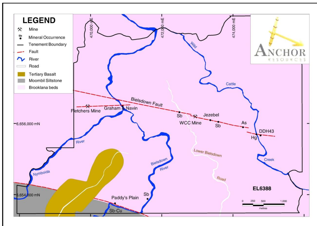
Figure 5 Bielsdown Project Geology
